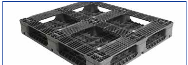
6-runner bottom deck allows for better stacking and racking capabilities.
